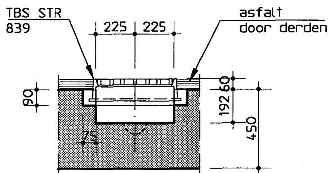
Detail a 1:20
