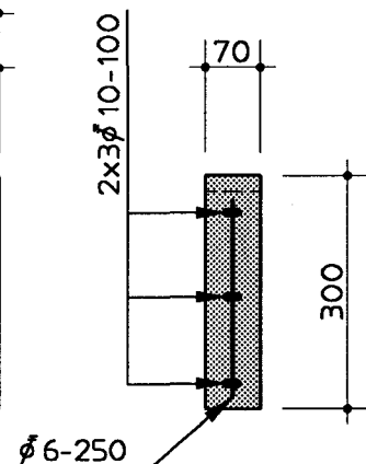
Dwarsdoorsn.
